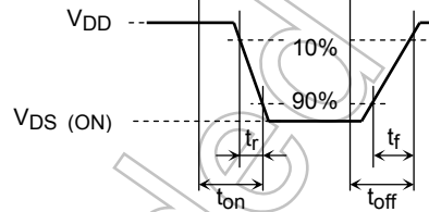
(c) V_{OUT}
