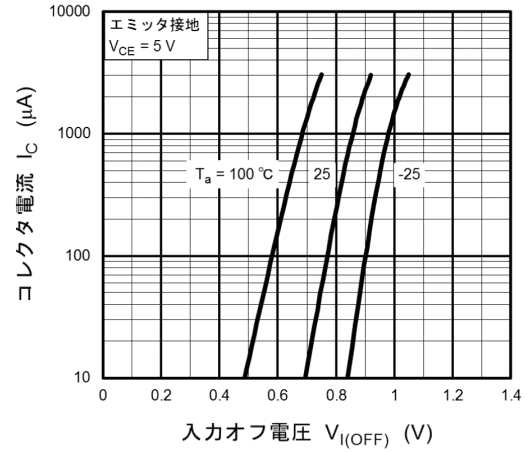
図 10.7 RN1115MFV I_C - V_{I(OFF)}
