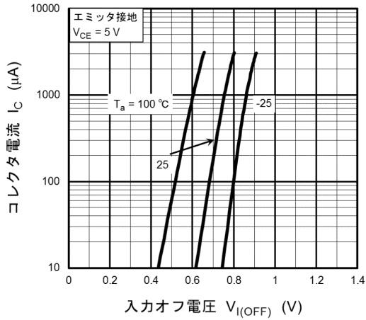
図 10.6 RN1114MFV I_C - V_{I(OFF)}
