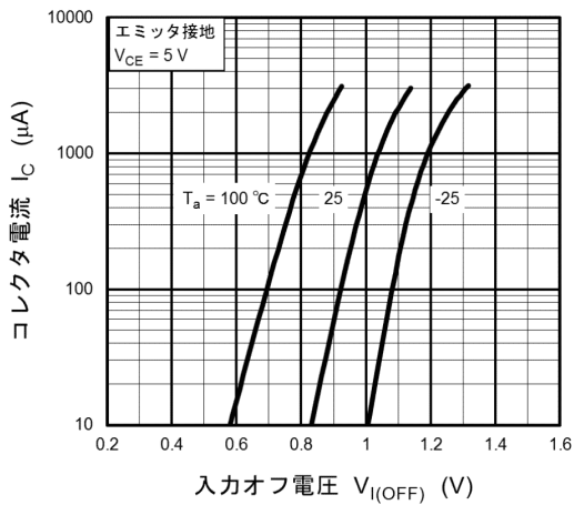
図 10.8 RN1116MFV I_C - V_{I(OFF)}
