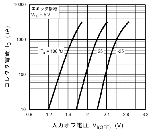
図 10.9 RN1117MFV I_C - V_{I(OFF)}
