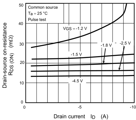
Fig. 7.5 R_{DS(ON)} - I_D
