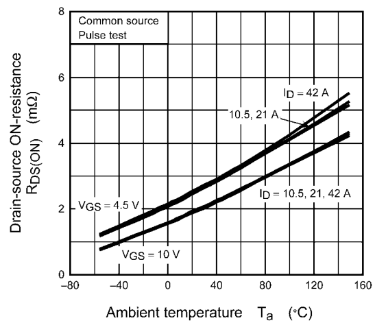
Fig. 8.6 R_{DS(ON)} - T_a
