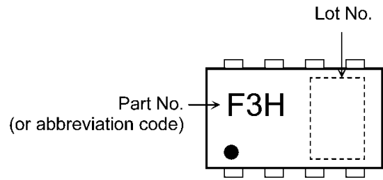
Fig. 7.1 Marking
