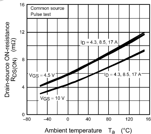
Fig. 8.6 R_{DS(ON)} - T_a
