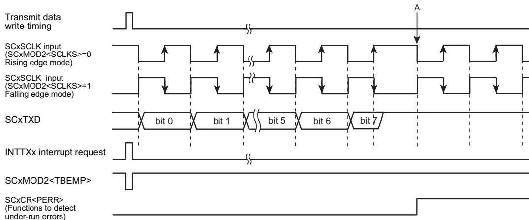
Figure 13-16 Transmit Operation in the I/O Interface Mode (Clock Input Mode)
