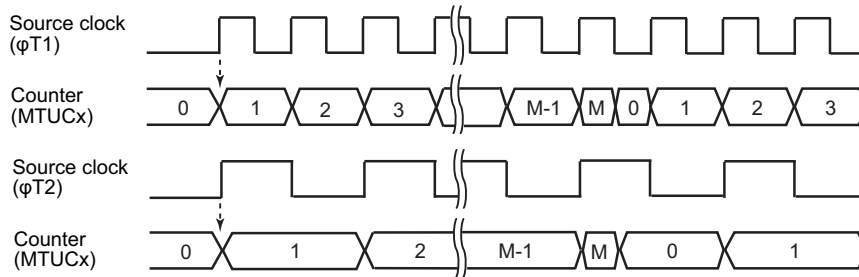
Figure 12-5 Count-up/clear operation when \phi T1 , \phi T2 or \phi T4 is selected as a source clock
