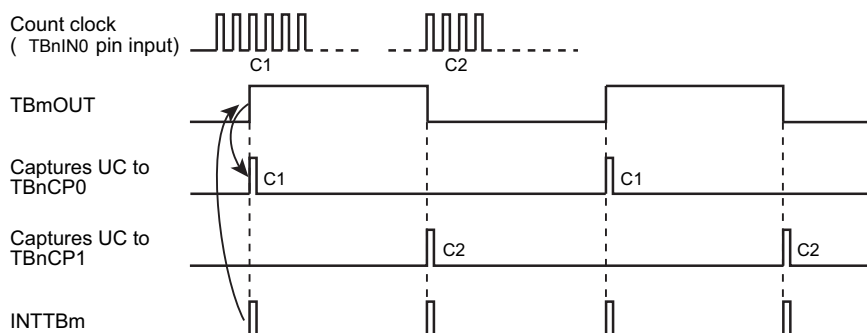
Figure 11-6 Frequency measurement
