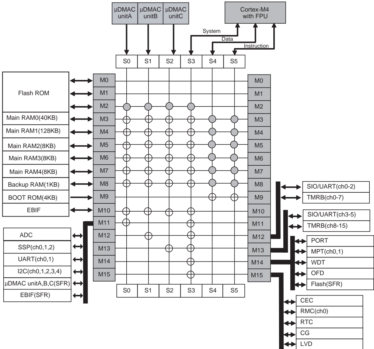
Figure 4-4 Bus Matrix of TMPM461F15/F10FG
