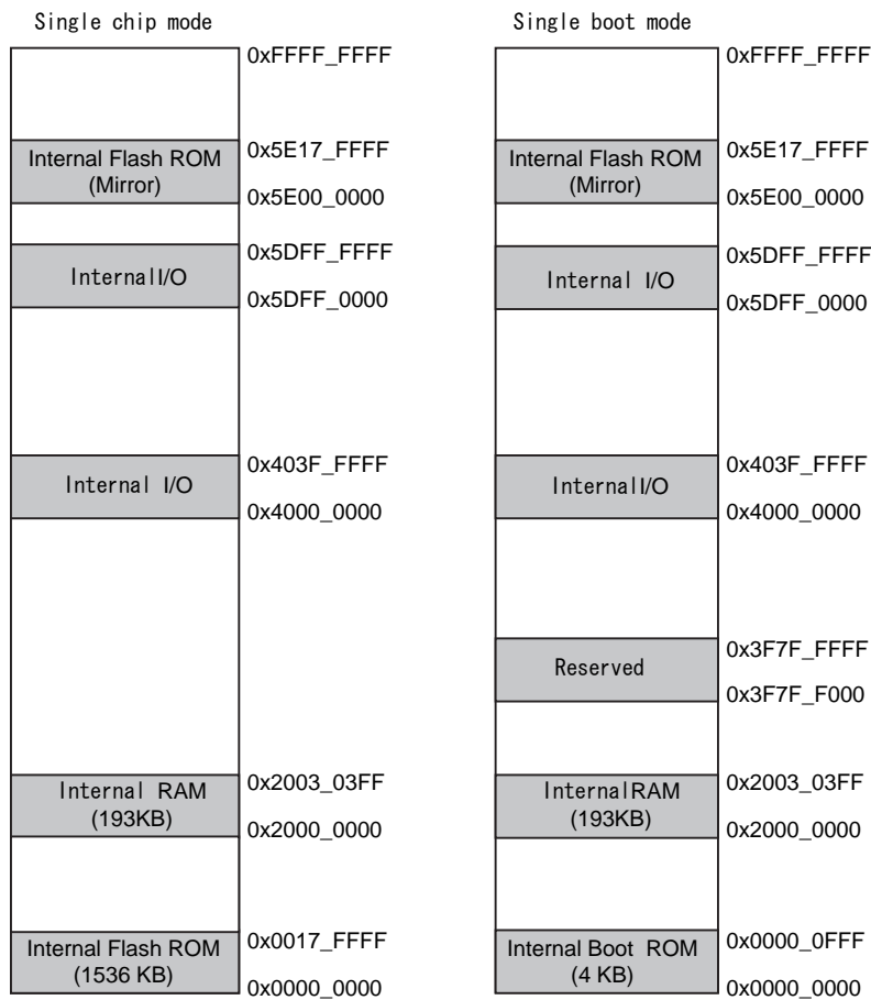
Figure 24-2 Comparison of memory map (TMPM461F15FG)
