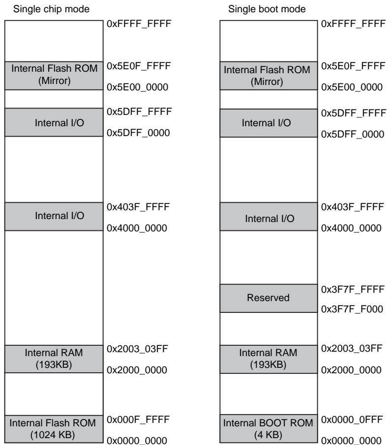
Figure 24-3 Comparison of memory map (TMPM461F10FG)
