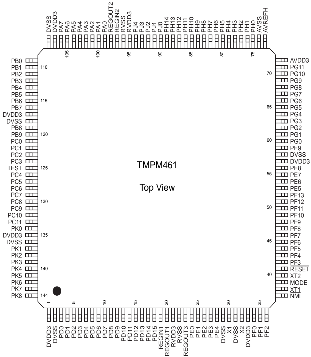
Figure 1-2 Pin Layout (LQFP144 TOP VIEW)
