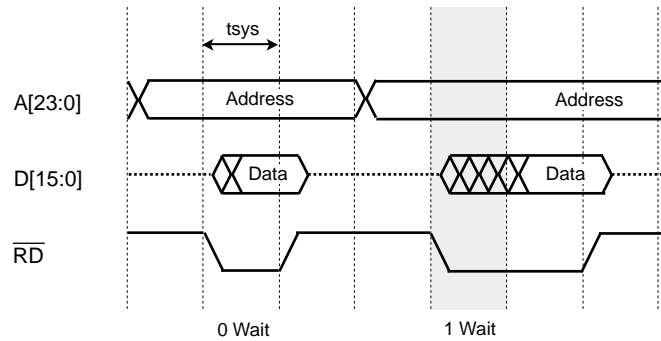
Figure 10-3 Read Operation Timing (Internal wait)
