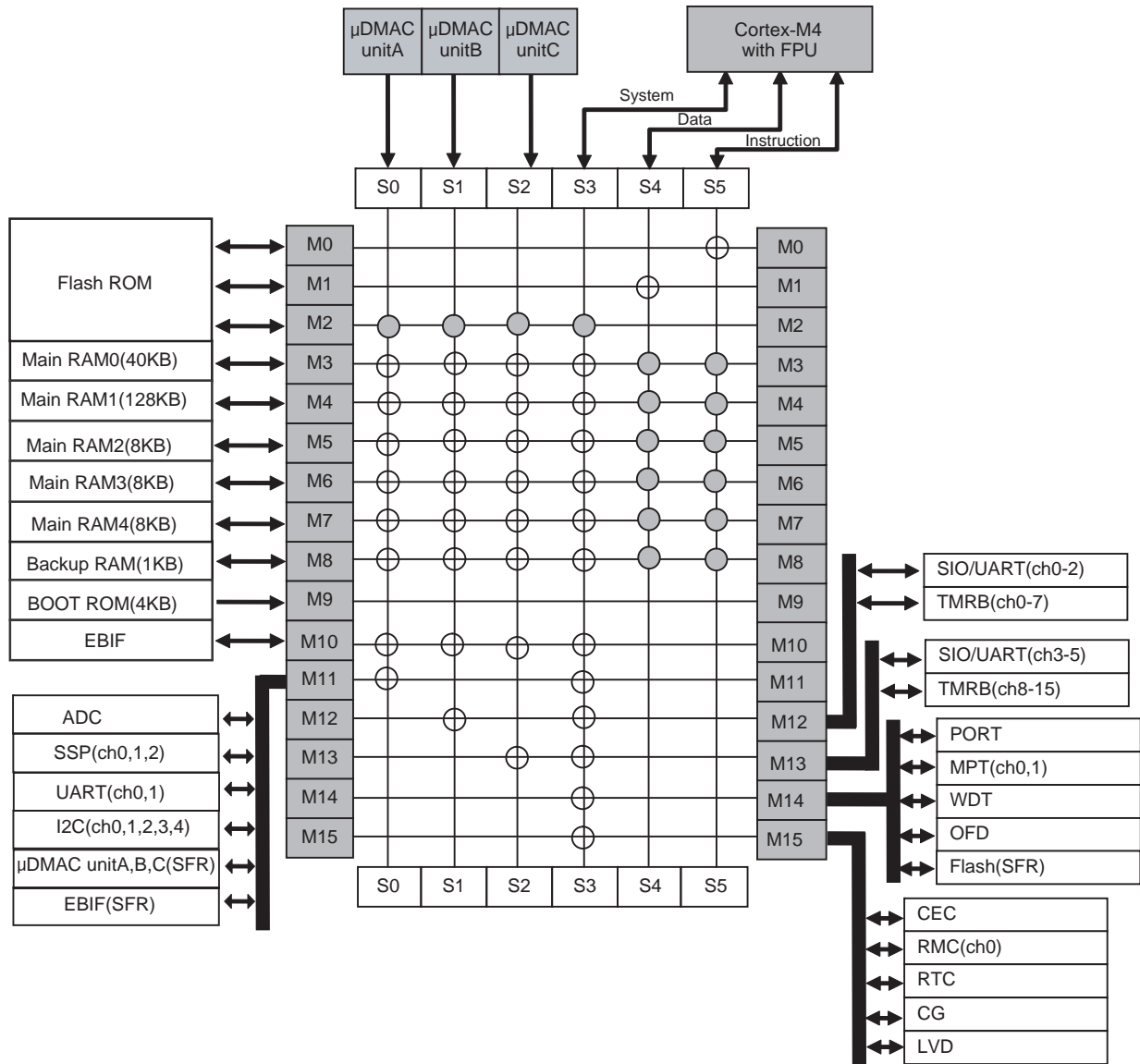
Figure 4-3 Bus Matrix of TMPM461F15/F10FG
