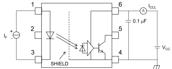
Fig. 13.1.4 I_{CCL} Test Circuit
