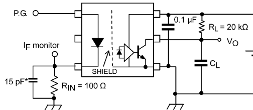
Fig. 13.1.6 Switching Time Test Circuit and Waveform
