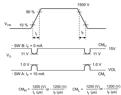
Fig. 13.1.7 Common-Mode Transient Immunity Test Circuit and Waveform
