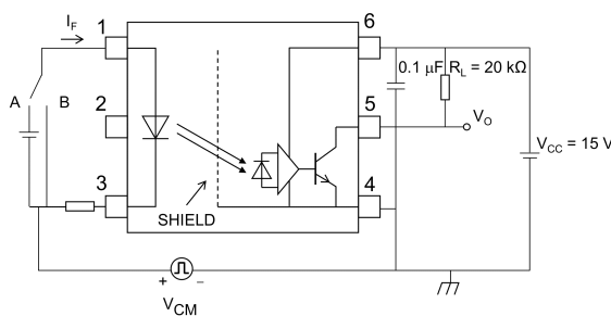
Fig. 13.1.7 Common-Mode Transient Immunity Test Circuit and Waveform
