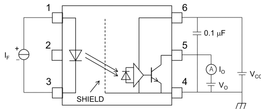
Fig. 13.1.5 I_O Test Circuit
