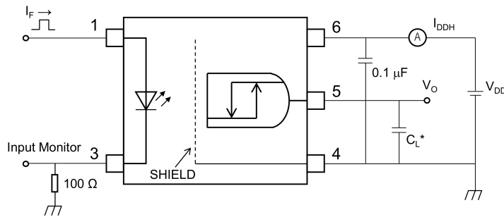
Fig. 12.1.6 Switching Time Test Circuit and Waveform
