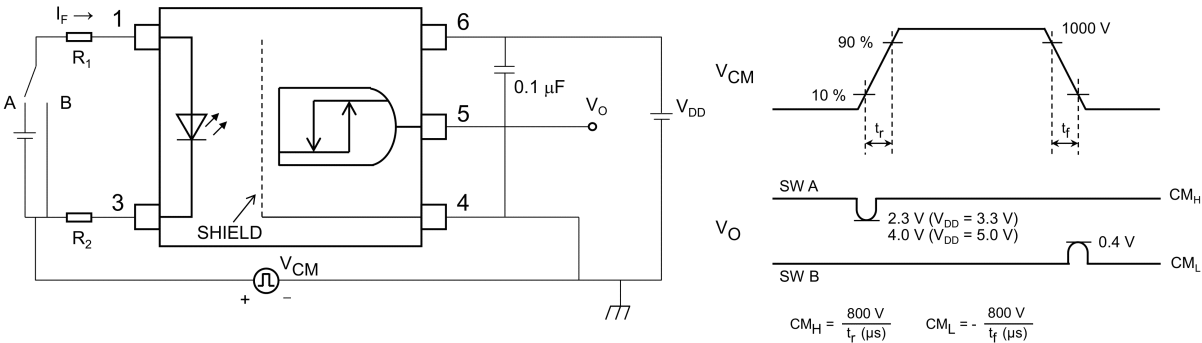
Fig. 12.1.7 Common-Mode Transient Immunity Test Circuit and Waveform
