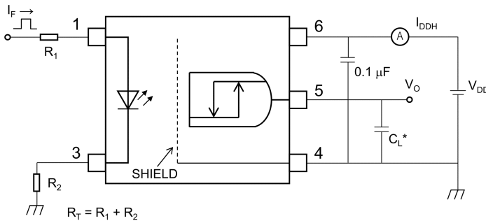
Fig. 12.1.5 Switching Time Test Circuit and Waveform
