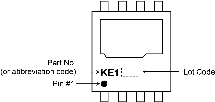
Fig. 7.1 Marking
