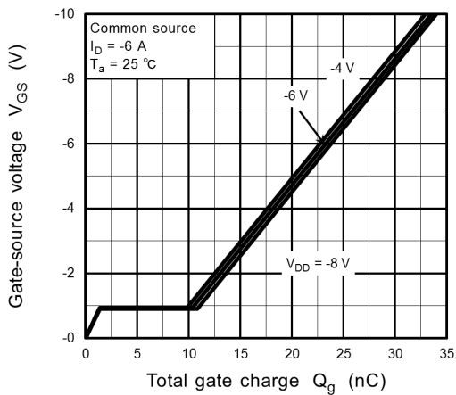
Fig. 9.11 Dynamic Input Characteristics
