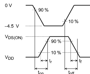
Fig. 6.3.2 Input Waveform/Output Waveform
