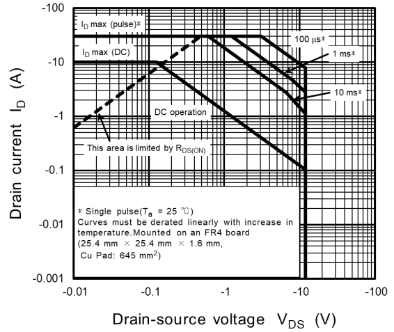
Fig. 9.14 Safe Operating Area
