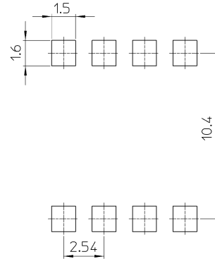
Fig. 14.2 Lead forming and taping option (LF4), (TP4)
