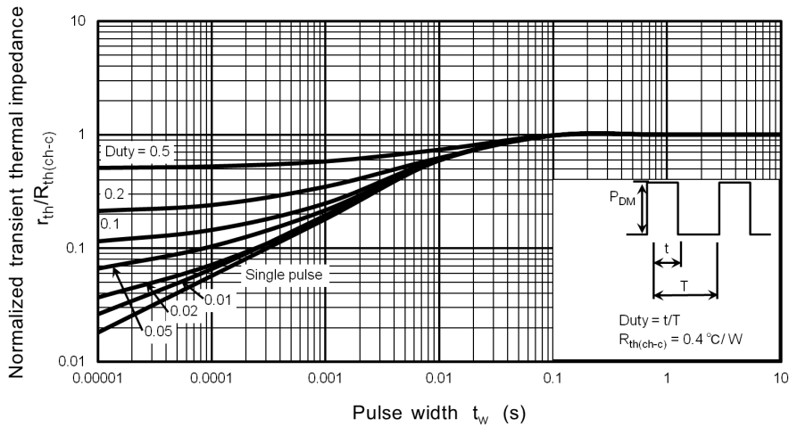
Fig. 9.13 r_{tr}/R_{th(ch-c)} - t_w (Guaranteed Maximum)
