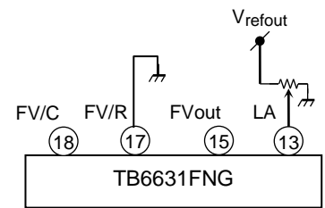
<Application circuit example>
