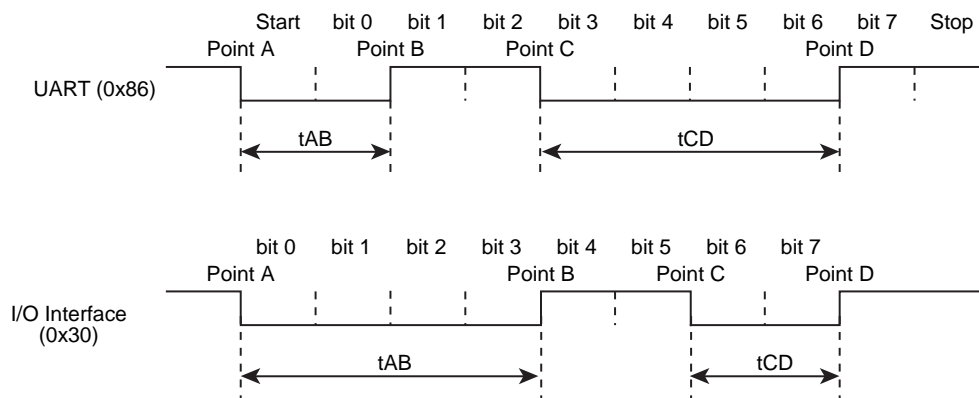
Figure 17-6 Serial operation mode determination data
