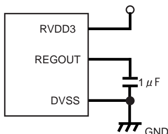
Figure 1-3 Capacitor for a regulator connection circuit
