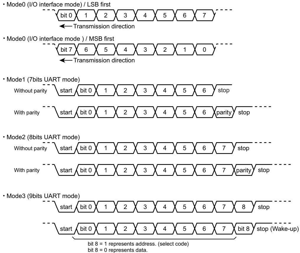
Figure 12-3 Data Format
