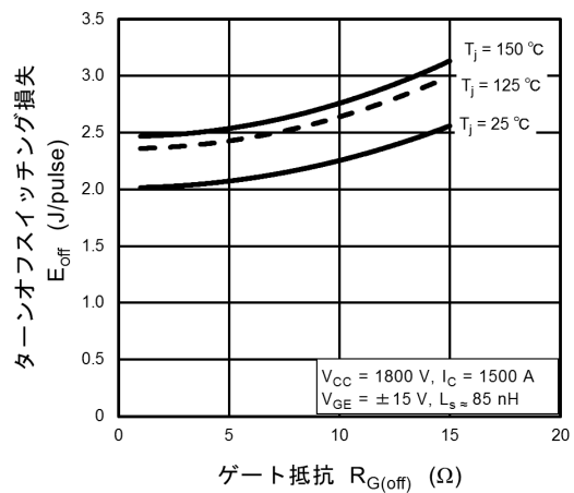
図 7.12 E_{off} - R_{G(off)}
