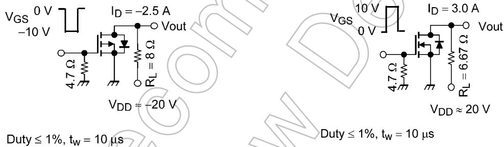
Fig. 6.2.1 Switching Time Test Circuit (P-ch) Fig. 6.2.2 Switching Time Test Circuit (N-ch)
