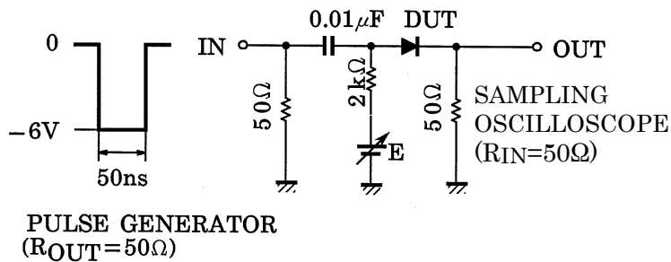
Fig.1 Reverse Recovery Time (t rr ) Test Circuit
