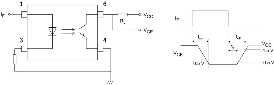
Fig. 10.1 Switching Time Test Circuit and Waveform
