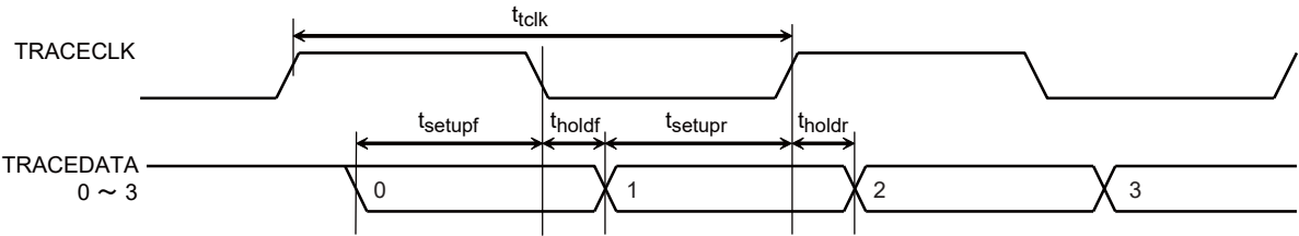
Figure 26-4 EMT trace timing
