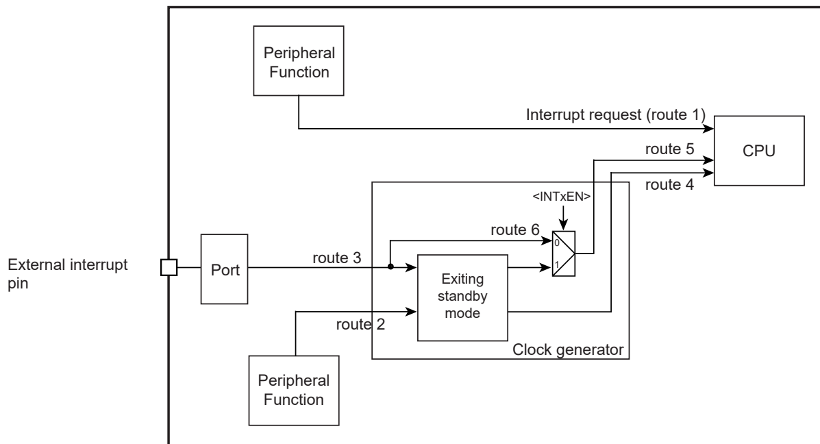
Figure 8-1 Interrupt Sources Route
