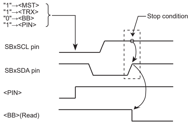
Figure 14-10 Generating the Stop Condition
