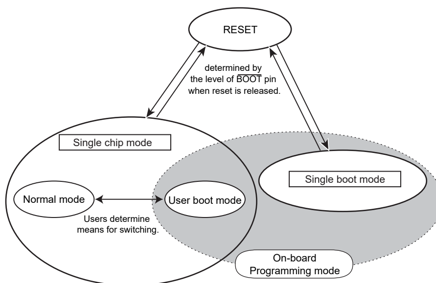
Figure 23-1 Mode transition
