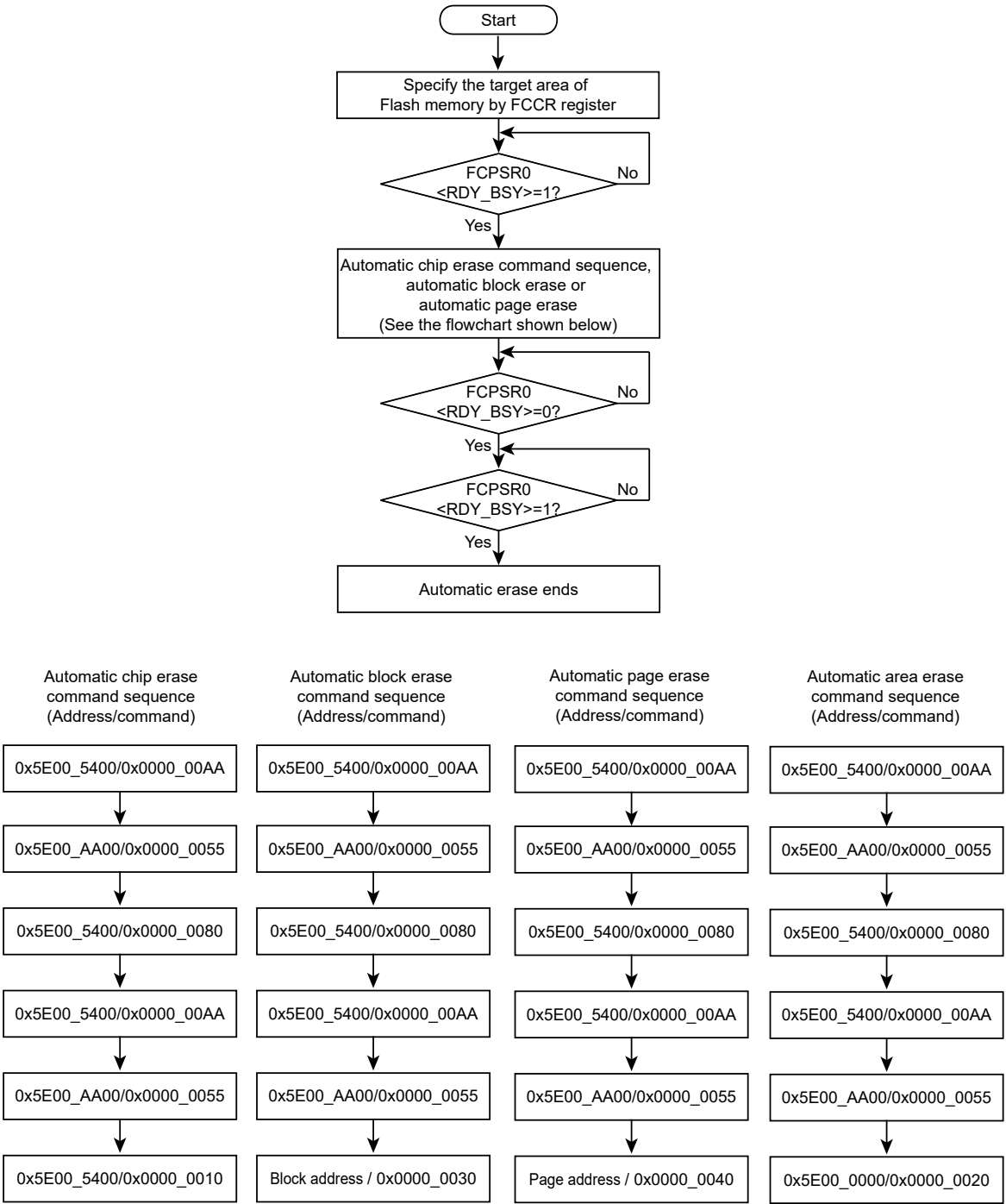
Figure 23-6 Flowchart of automatic erase
