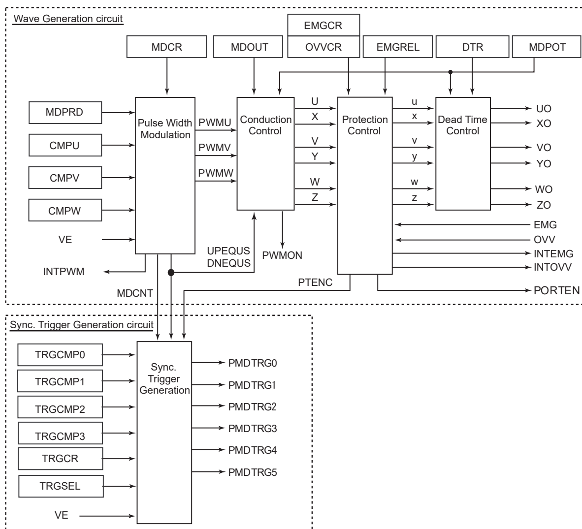
Figure 16-3 Block diagram of PMD Circuit
