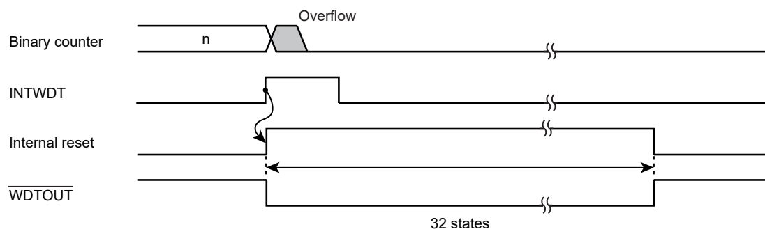
Figure 22-3 Internal reset generation
