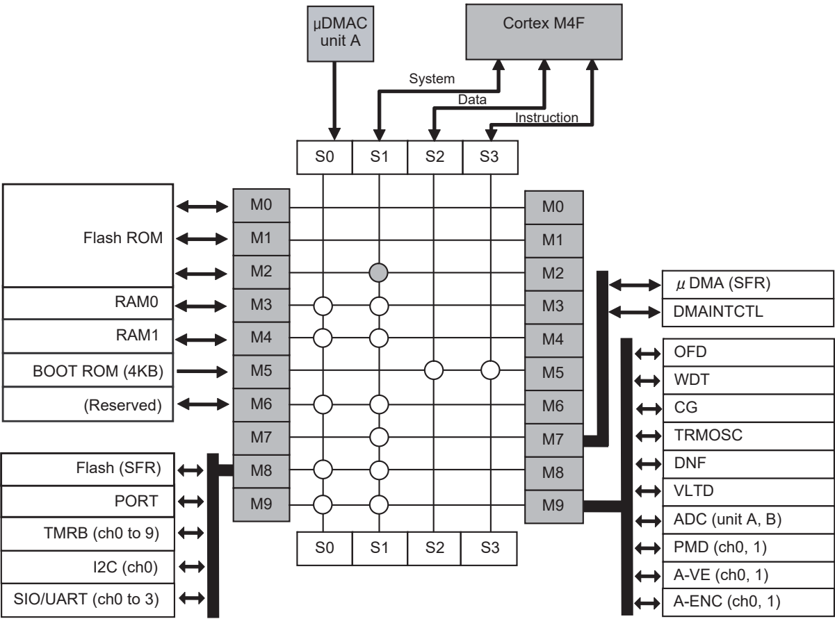
Figure 4-5 Bus Matrix of TMPM470FDFG/FZFG/FYFG
