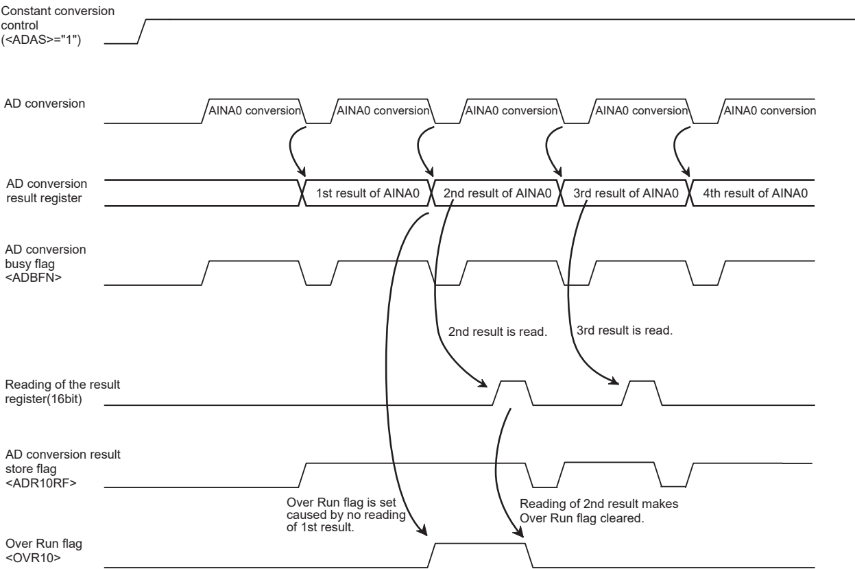
Figure 15-6 Constant conversion
