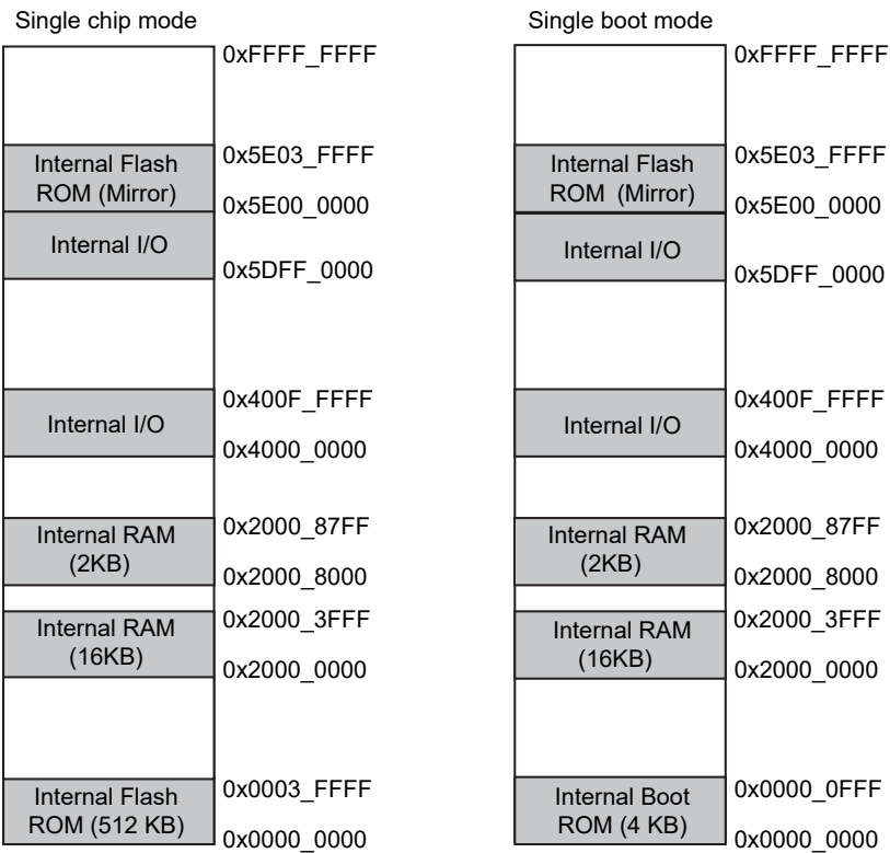
Figure 23-4 Comparison of memory map (TMPM470FYFG)
