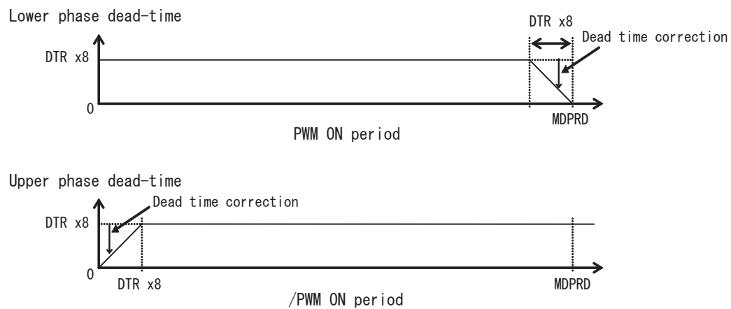
Figure 16-11 Dead Time correction
