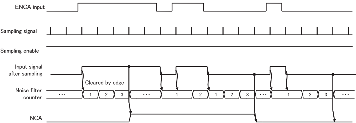
Figure 18-5 Noise cancelling (Continuous, <NCT>=3)
