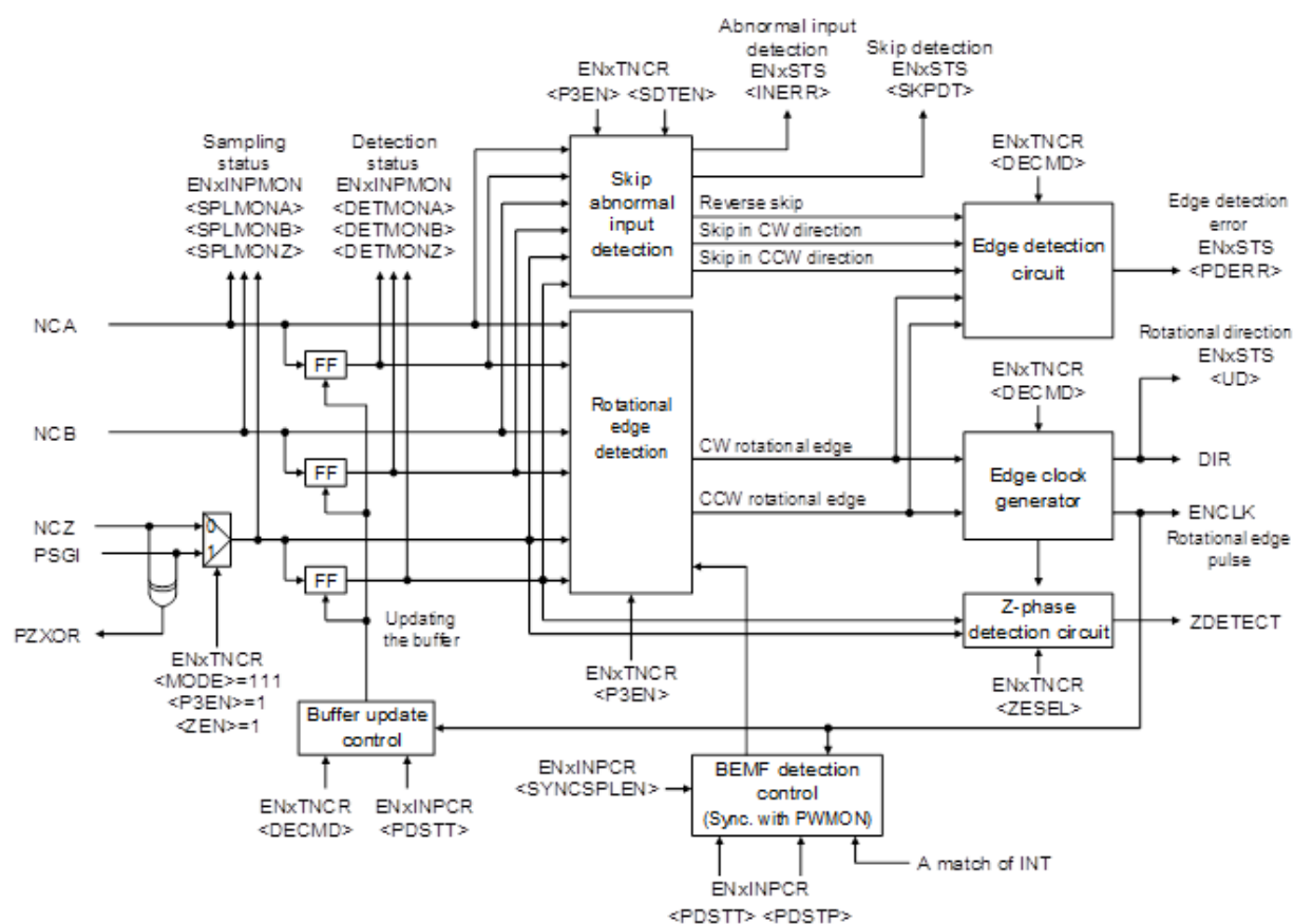
Figure 18-8 Configuration of the decoder
