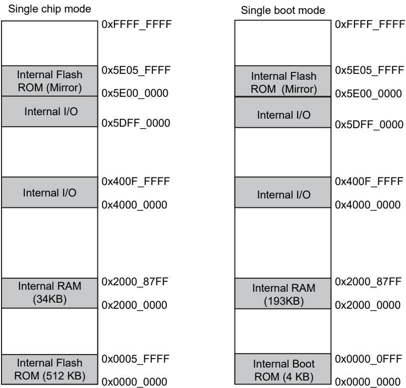
Figure 23-3 Comparison of memory map (TMPM470FZFG)
