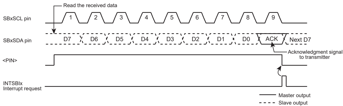
Figure 14-8 <BC[2:0]>= "000", <ACK>= "1" (Receiver Mode)
