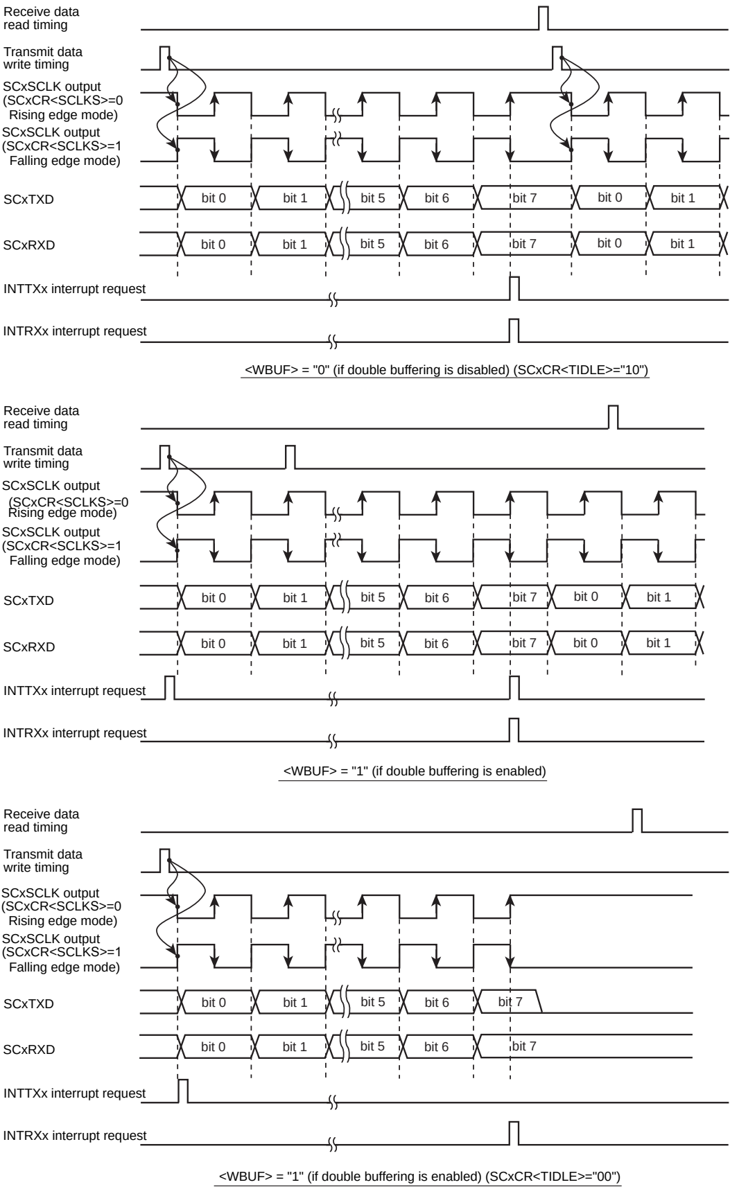
Figure 13-19 Transmit/Receive Operation in the I/O Interface Mode (SCLK Output Mode)
