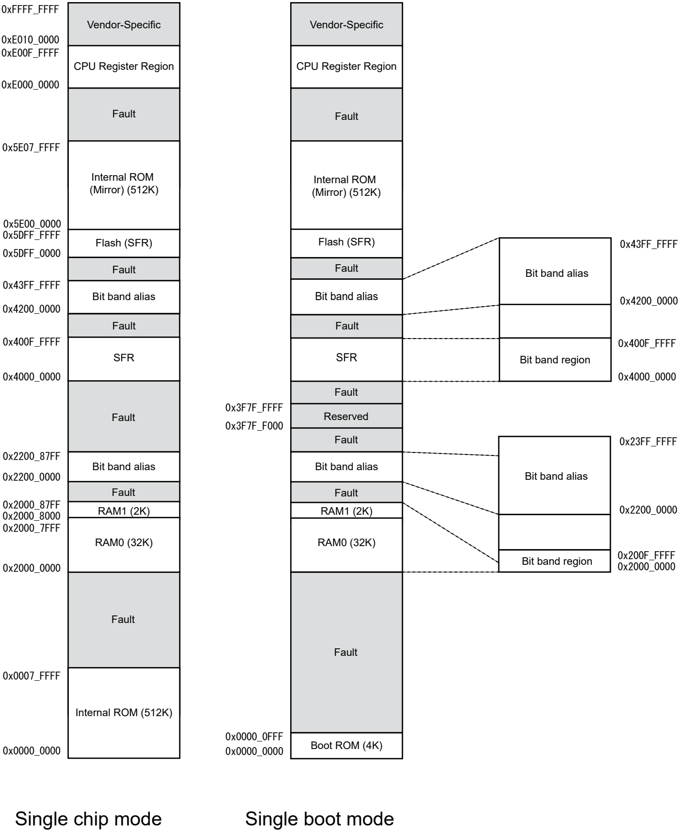
Figure 4-1 MemoryMap(512KB)
