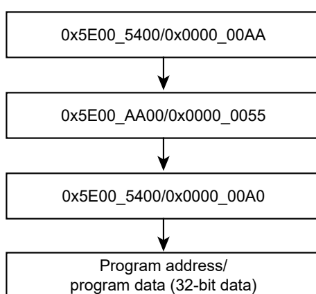
Figure 23-5 Flowchart of Automatic Program
