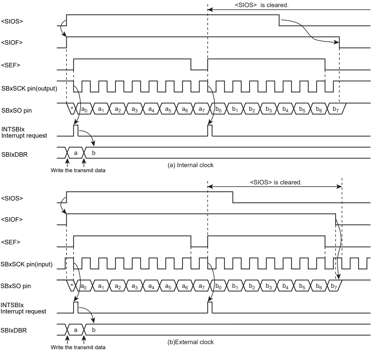
Figure 14-16 Transmit Mode
