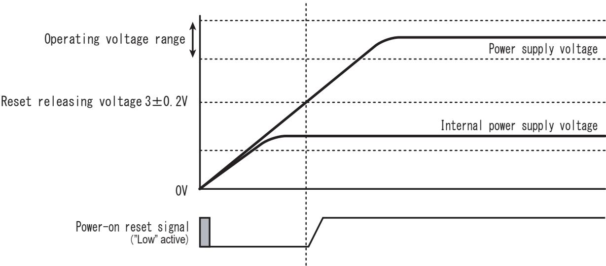
Figure 19-2 Power-on-reset operation timing at power-on
