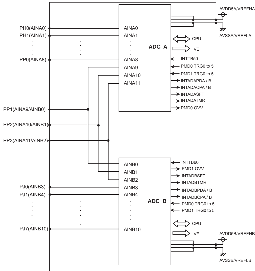
Figure 15-1 AD converters Block Diagram
