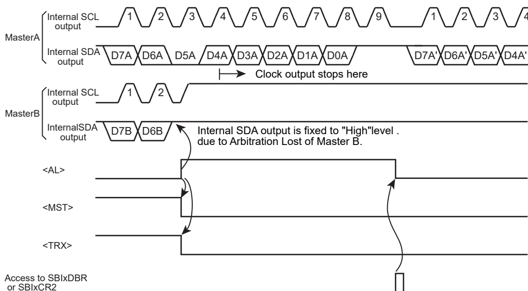
Figure 14-5 Example of Master B Lost Arbitration ( \text{D7A} = \text{D7B} , \text{D6A} = \text{D6B} )
