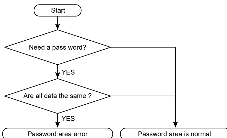
Figure 23-11 Password area check flow chart
