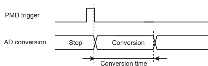
Figure 17-7 ADC conversion time
