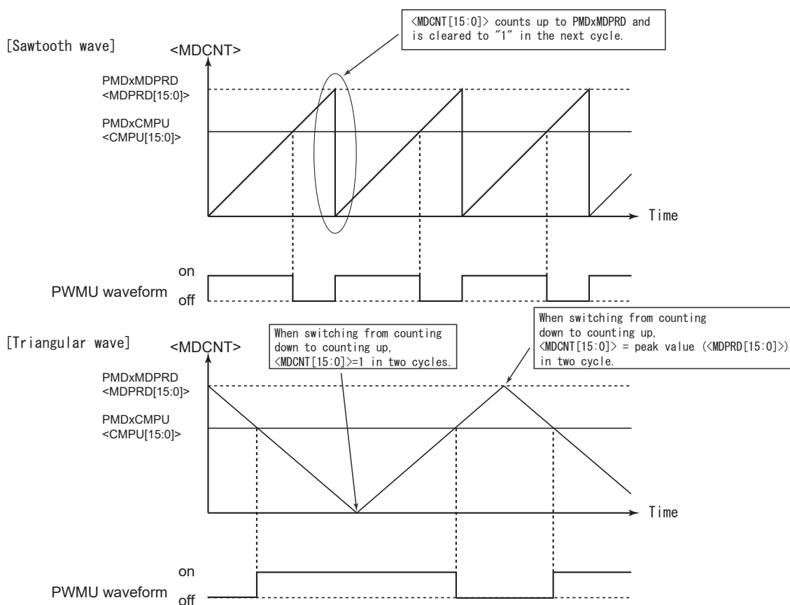
Figure 16-5 PWM Waveforms
