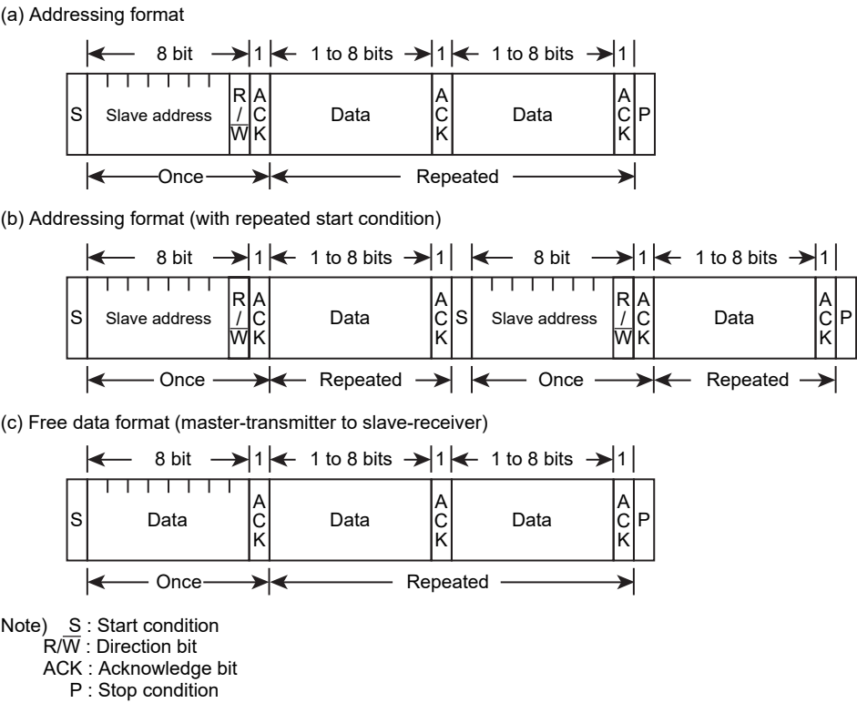
Figure 14-12 I2C Bus Mode Data Formats
