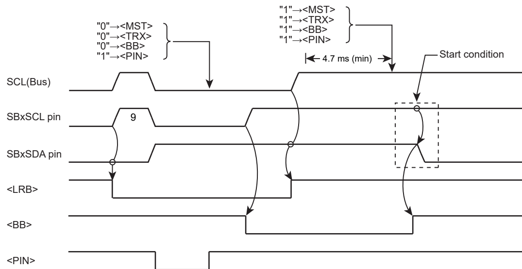
Figure 14-11 Timing Chart of Generating a Restart
