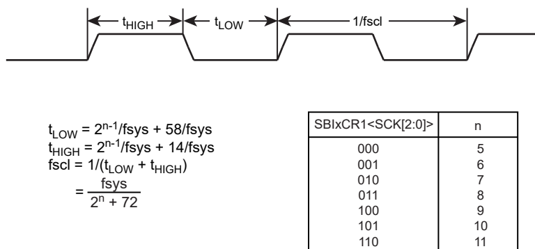
Figure 14-2 Clock source
