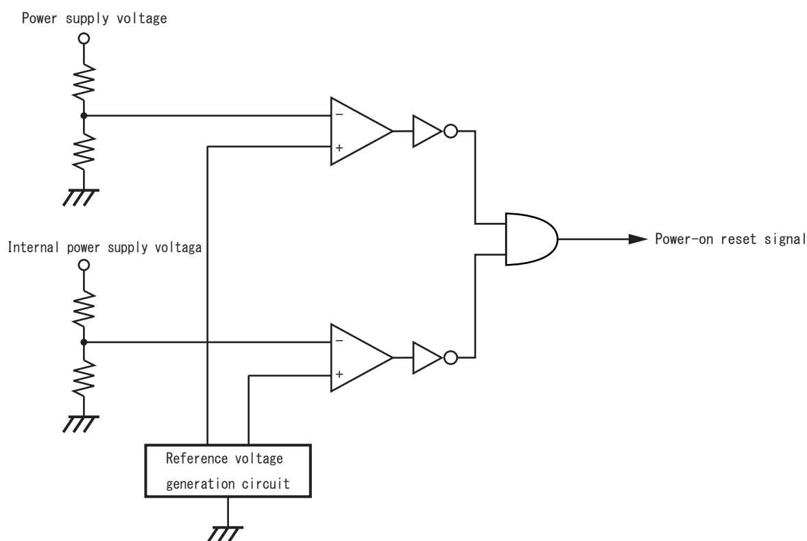
Figure 19-1 Power-on-reset circuit
