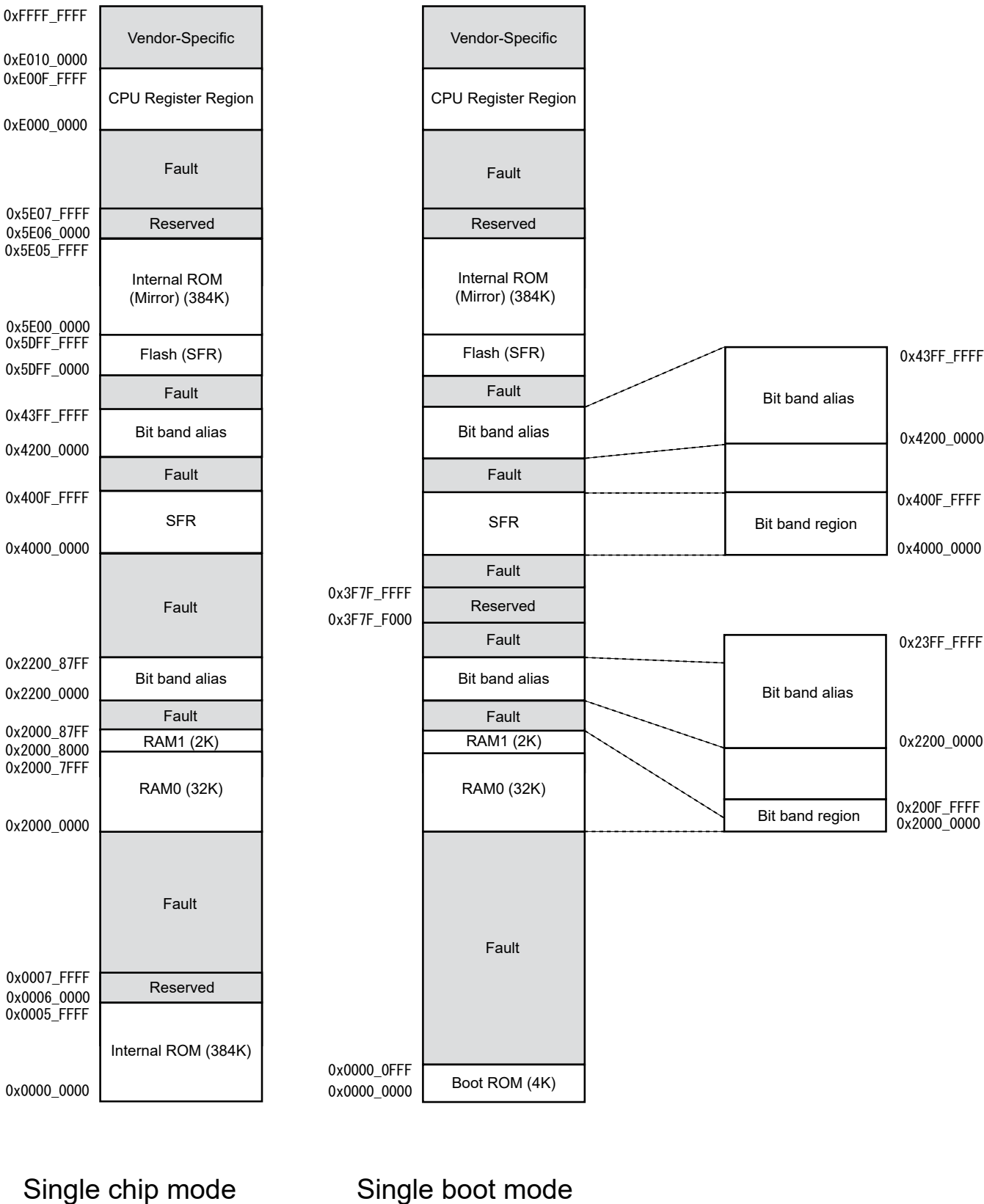
Figure 4-2 MemoryMap(384KB)
