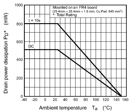
Fig. 7.12 P_D - T_a
