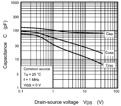
Fig. 7.8 C - VDS
