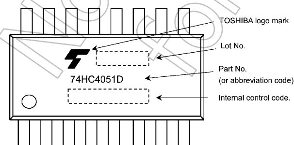
74HC4051D
