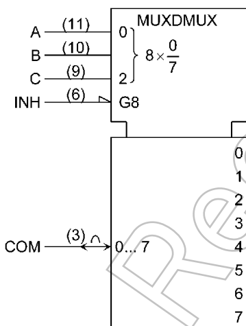
74HC4051D
