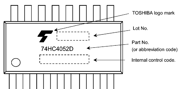
74HC4052D
