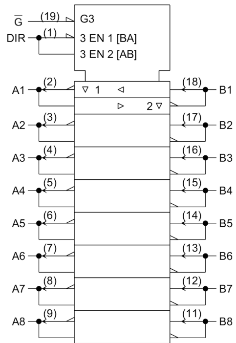
TC74ACT640P
