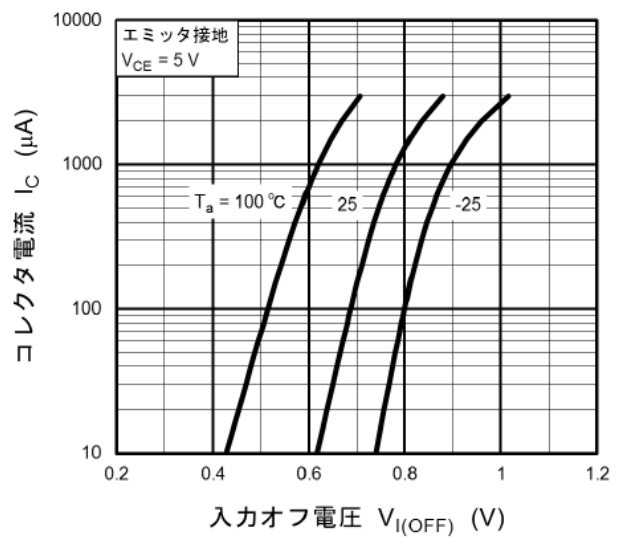
図 11.12 RN1106MFV I_C - V_{I(OFF)}
