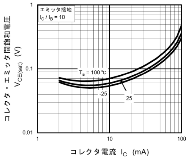
図 11.20 RN1102MFV V_{CE(sat)}-I_C
