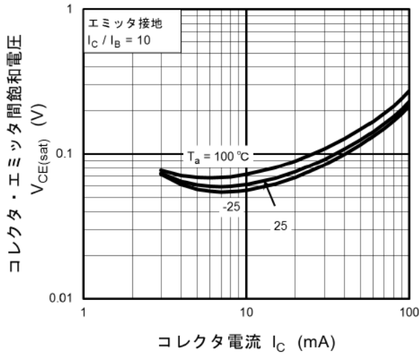
図 11.19 RN1101MFV V_{CE(sat)}-I_C
