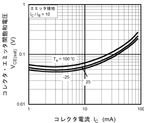
図 11.21 RN1103MFV V_{CE(sat)}-I_C
