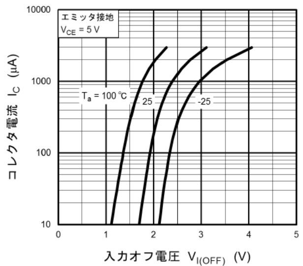
図 11.6 RN1109MFV I_C - V_{I(OFF)}
