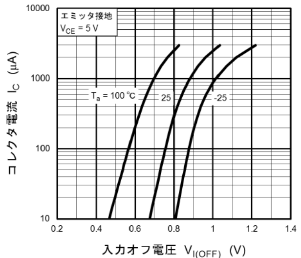
図 11.4 RN1107MFV I_C - V_{I(OFF)}
