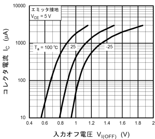
図 11.5 RN1108MFV I_C - V_{I(OFF)}
