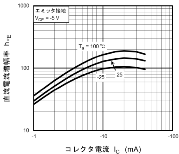
図 11.15 RN2103MFV h_{FE}-I_C
