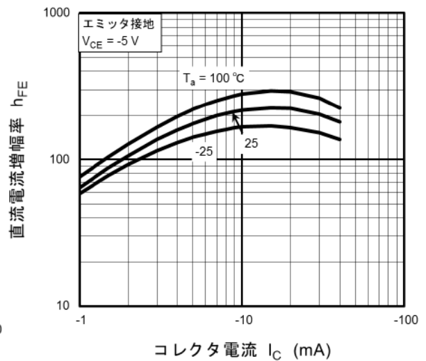
図 11.18 RN2106MFV h_{FE}-I_C
