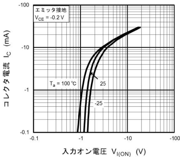
図 11.3 RN2103MFV I_C - V_{I(ON)}
