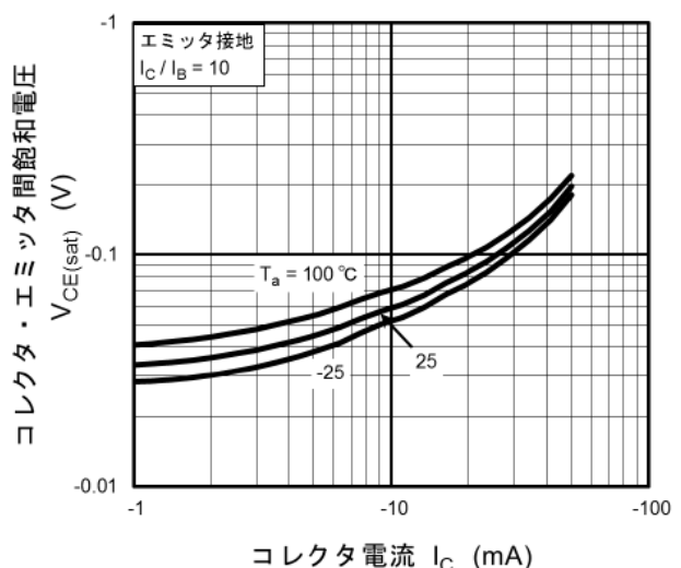
図 11.22 RN2104MFV V_{CE(sat)}-I_C
