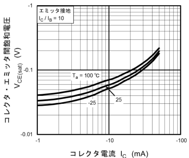
図 11.22 RN2104MFV V_{CE(sat)}-I_C
