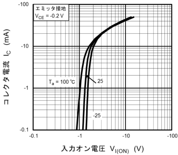
図 11.1 RN2101MFV I_C - V_{I(ON)}
