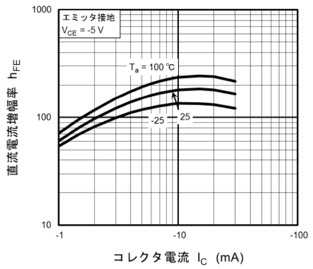
図 11.16 RN2104MFV h_{FE}-I_C
