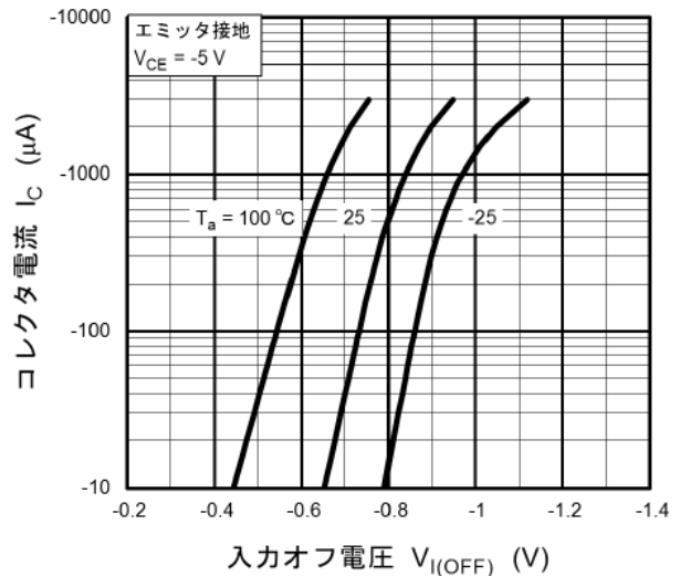
図 11.4 RN2107MFV I_C - V_{I(OFF)}
