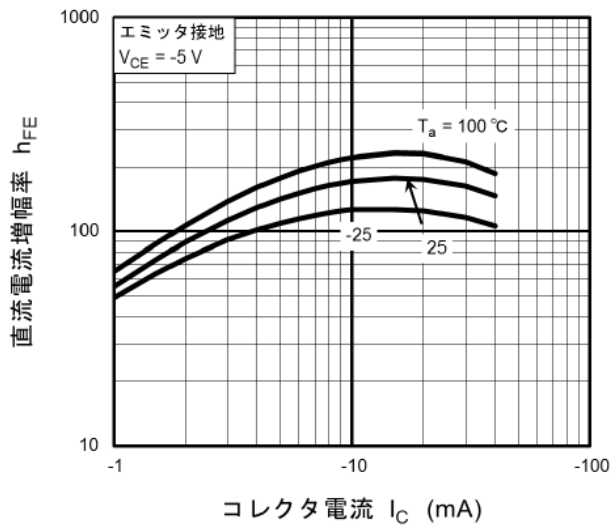
図 11.7 RN2107MFV h_{FE}-I_C
