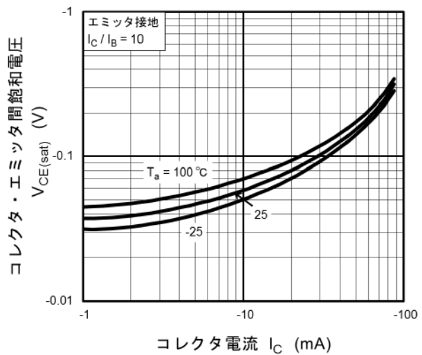
図 11.11 RN2108MFV V_{CE(sat)}-I_C
