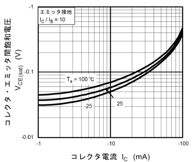
図 11.10 RN2107MFV V_{CE(sat)}-I_C
