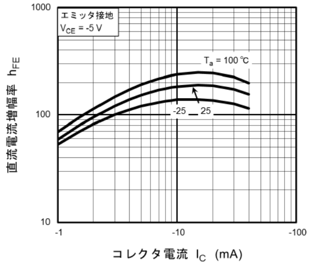
図 11.8 RN2108MFV h_{FE}-I_C
