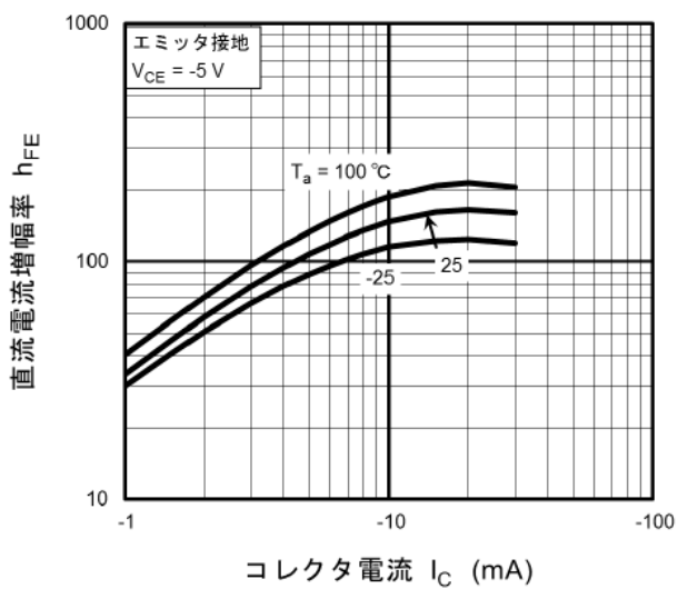
図 11.9 RN2109MFV h_{FE}-I_C
