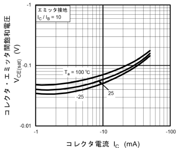
図 11.12 RN2109MFV V_{CE(sat)}-I_C
