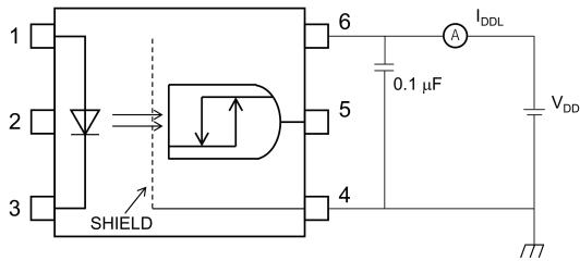
Fig. 12.1.3 I_{DDL} Test Circuit
