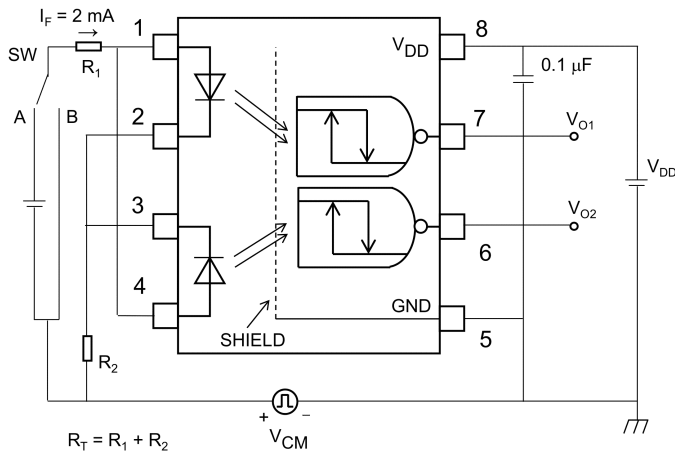
Fig. 12.1.6 Common-Mode Transient Immunity Test Circuit and Waveform
