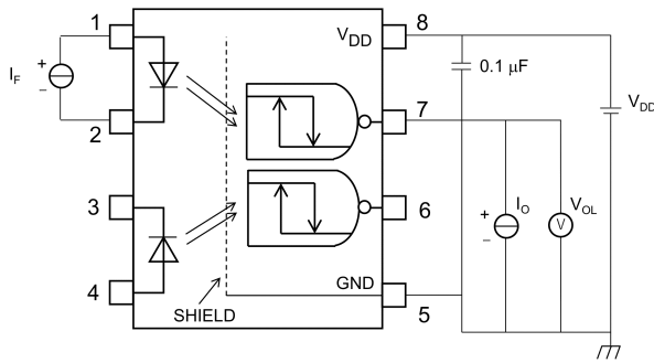
Fig. 12.1.1 V_{OL} Test Circuit
