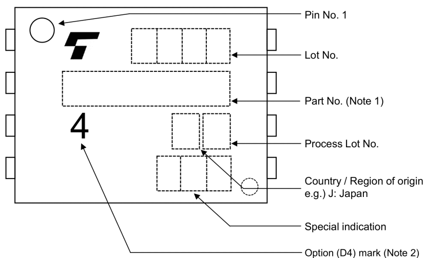
Fig. 16.4 Marking Example
