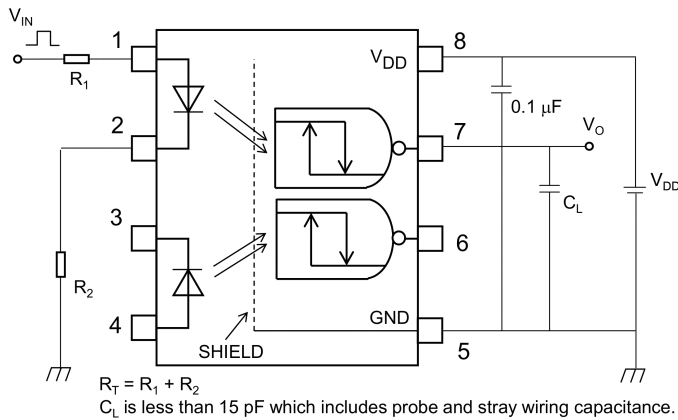
Fig. 12.1.5 Switching Time Test Circuit and Waveform
