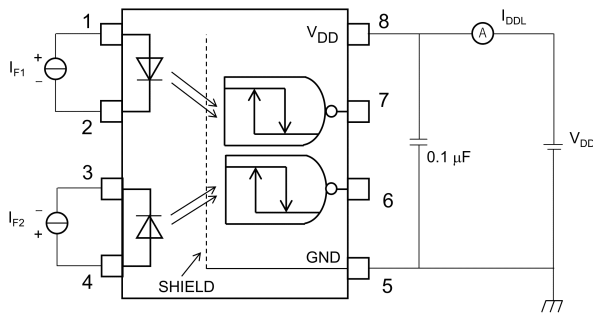
Fig. 12.1.3 I_{DDL} Test Circuit
