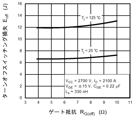
図 7.9 E_{off} - R_{G(off)}
