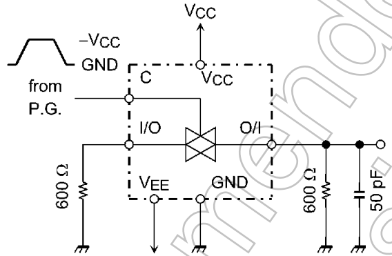
Figure 4 Feedthrough Attenuation
