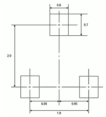
SOT23 (Unit: mm)
