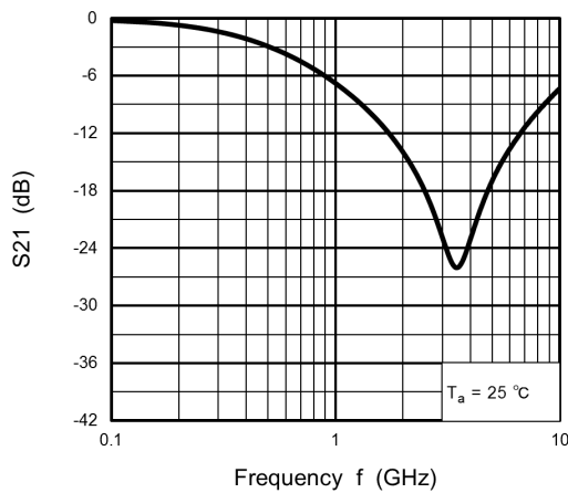
図 8.5 S_{21} - f
