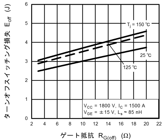
図 7.10 E_{off} - R_{G(off)}
