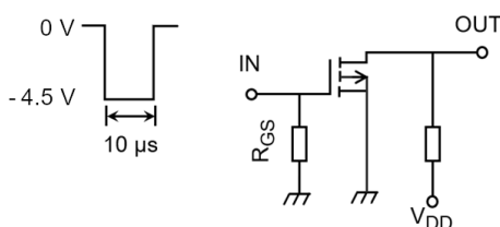
Fig. 5.3.1 Switching Time Test Circuit
