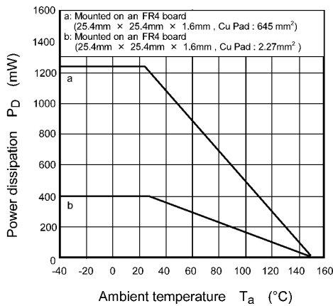
Fig. 8.11 P_D - T_a
