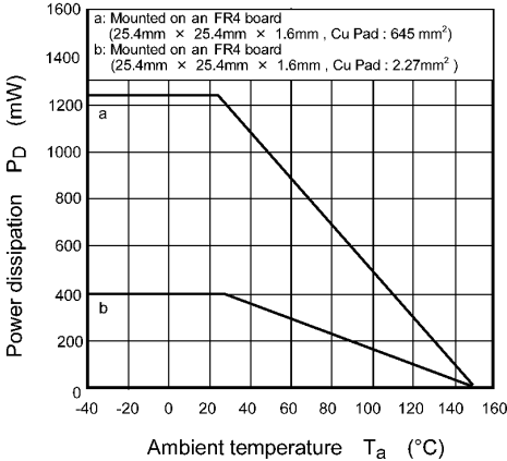
Fig. 8.13 P_D - T_a
