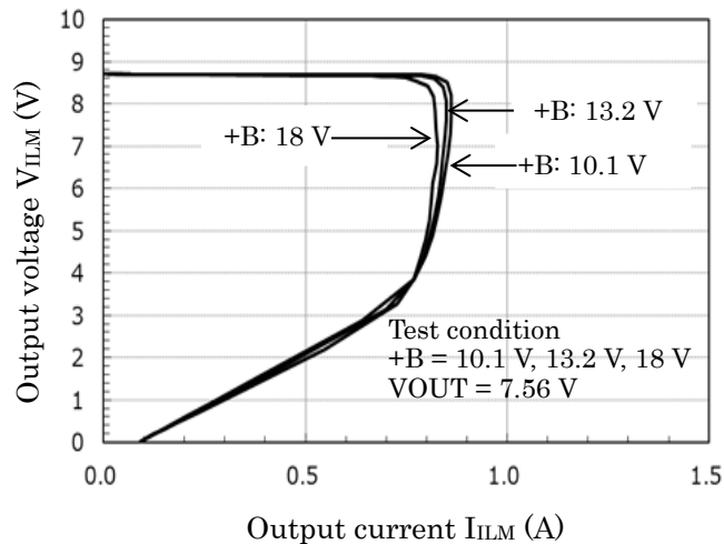
V_{ILM} - I_{ILM} (8.5 V setting)
