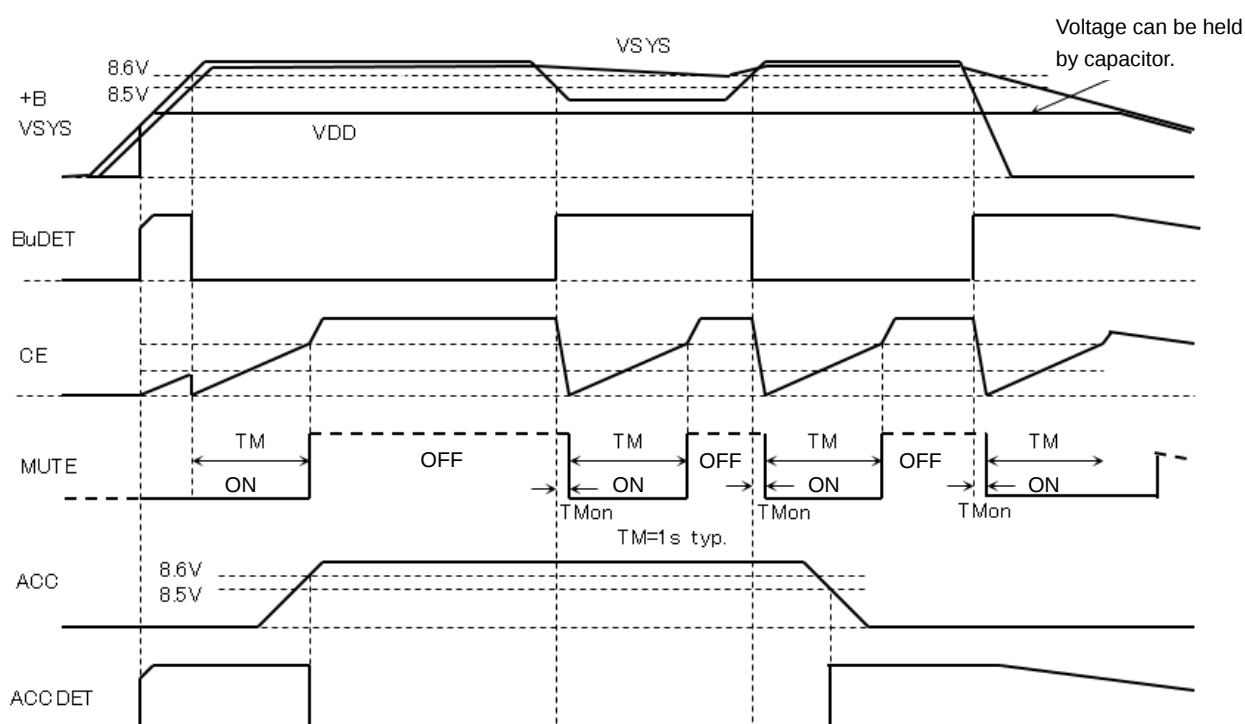
Timing chart
