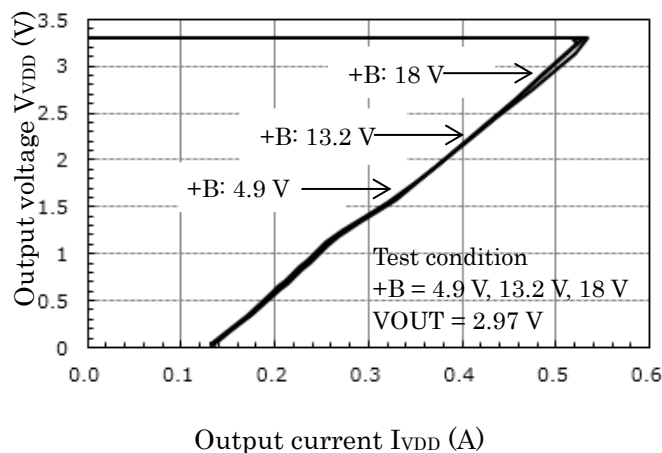
V_{VDD} - I_{VDD}
