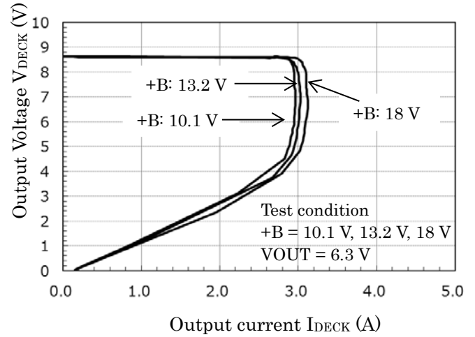
V_{DECK}-I_{DECK} (8.5 V setting)
