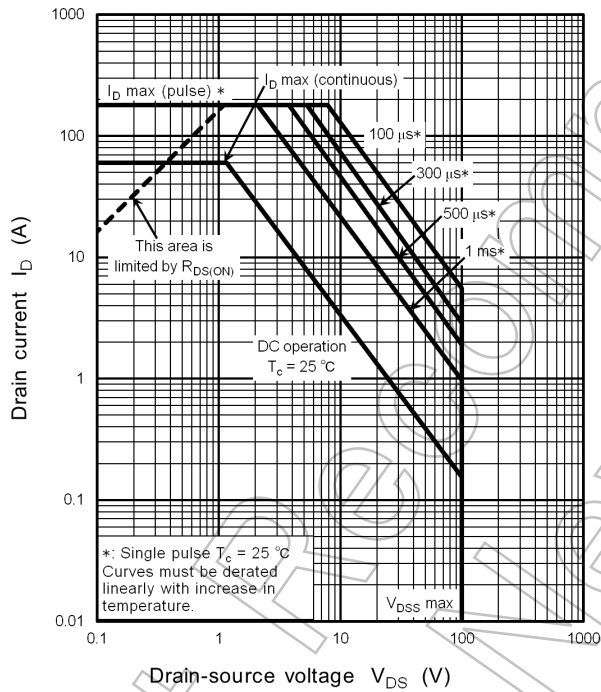
Fig. 9.19 Safe Operating Area (Guaranteed Maximum)
