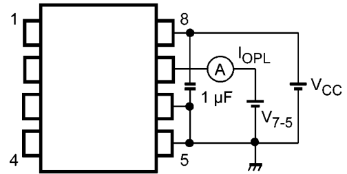
Fig. 12.1.2 I_{OPL} Test Circuit
