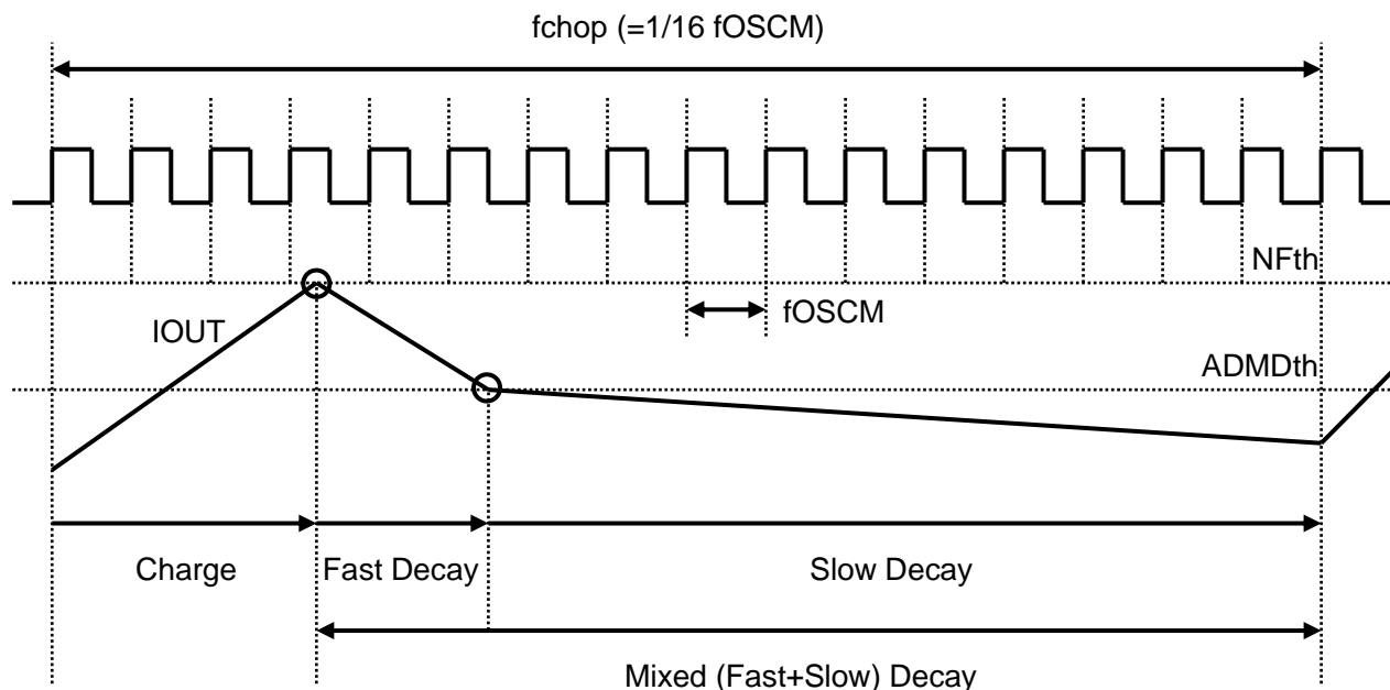
図 7.4 ADMD(Advanced Dynamic Mixed Decay)定電流制御
