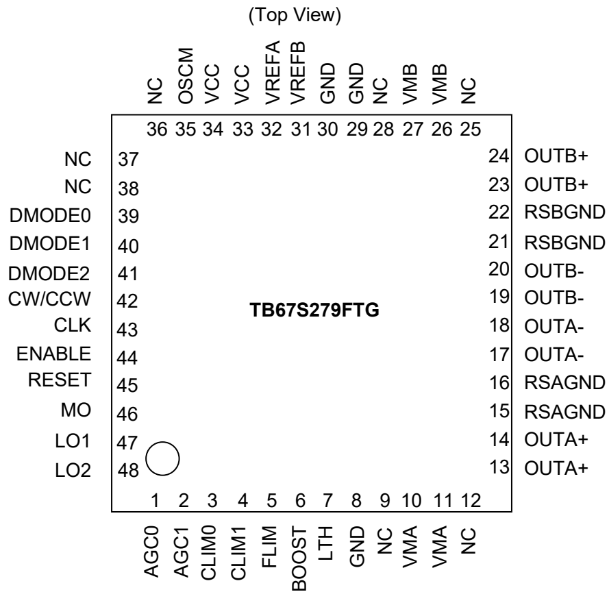
Figure 3.1 Pin Assignments
