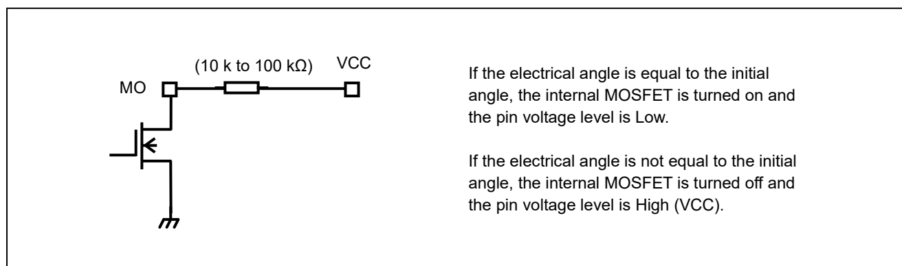
Figure 7.1 MO function Equivalent Circuit
