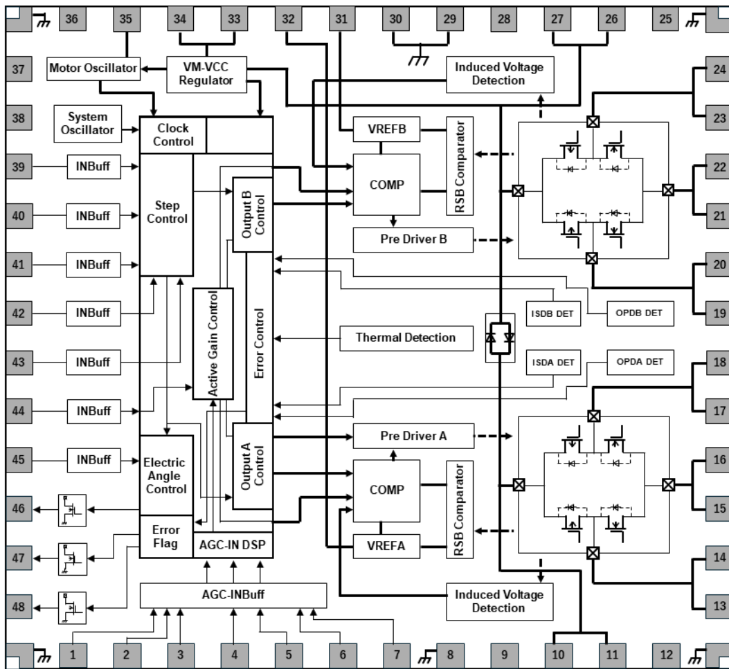
Figure 5.1 Block diagram
