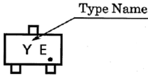
Fig. 10.5 Marking RN2105MFV
