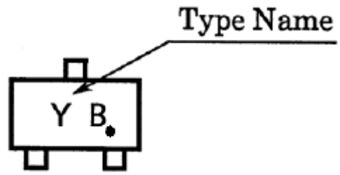
Fig. 10.2 Marking RN2102MFV
