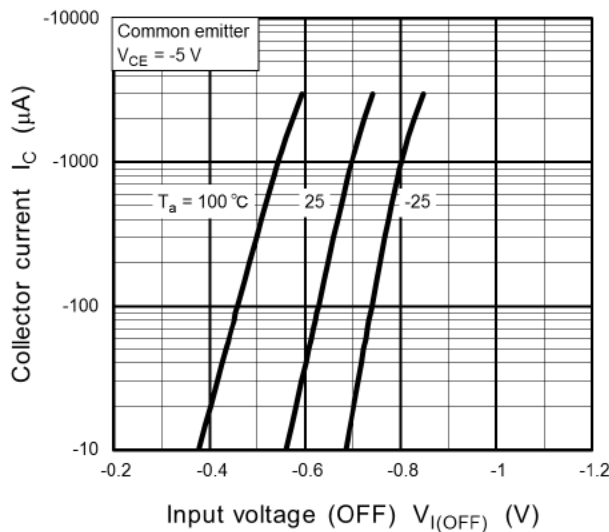
Fig. 11.11 RN2105MFV I_C - V_{I(OFF)}
