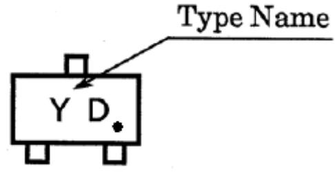
Fig. 10.4 Marking RN2104MFV
