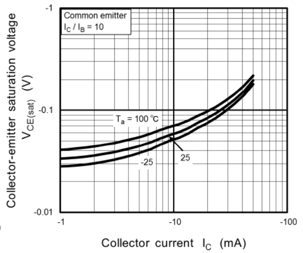
Fig. 11.22 RN2104MFV V_{CE(sat)} - I_C
