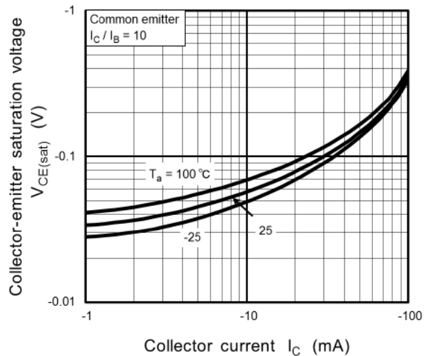
Fig. 11.24 RN2106MFV V_{CE(sat)} - I_C
