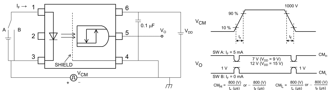
Fig. 12.1.8 Common-Mode Transient Immunity Test Circuit and Waveform
