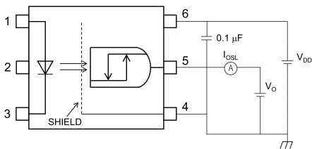
Fig. 12.1.5 I_{OL} Test Circuit
