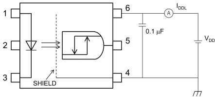
Fig. 12.1.3 I_{CCL} Test Circuit
