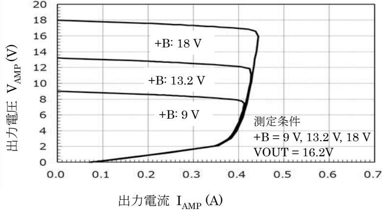
V_{AMP}-I_{AMP}
