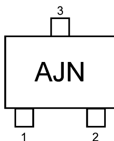
Fig. 7.1 Marking
